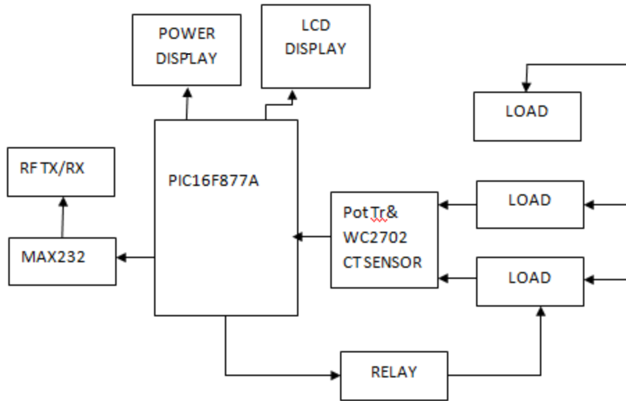
Fig3.1.Receiver side
