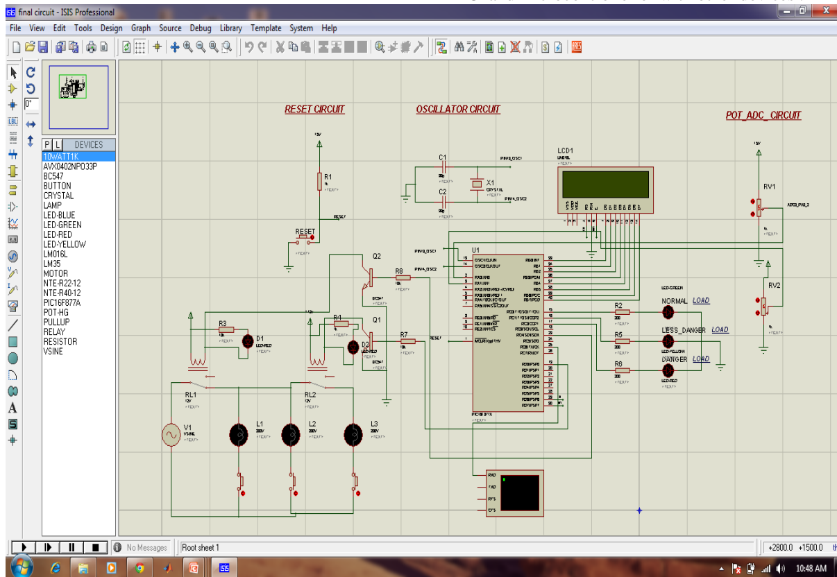
Fig 3.3.Circuit Diagram
