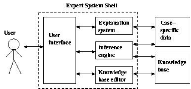
Figure 1: Architecture of an Expert System
