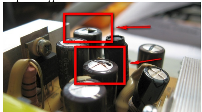
Figure 4: The figure shows the Power Supply Failure [3]
