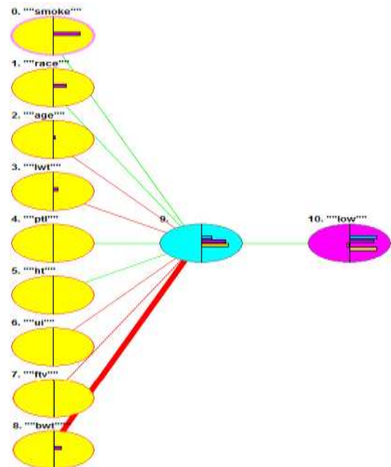
Figure 1: Shows the Design of the Neural Networks
