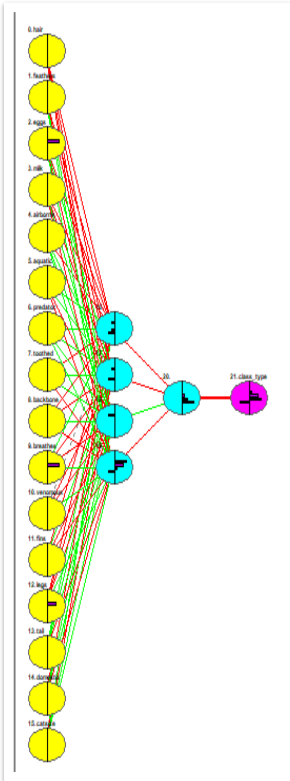
Figure 2: Animal Classification ANN
