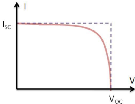
Figure 3 - Illuminated I-V Sweep Curve Short Circuit Current ( I_{SC} )
