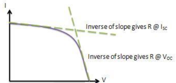
Figure 7 - Obtaining Resistances from the I-V Curve
