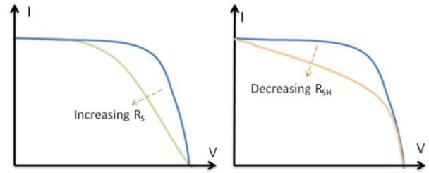
Figure 6 - Effect of Diverging R_S & R_{SH} From Ideality
