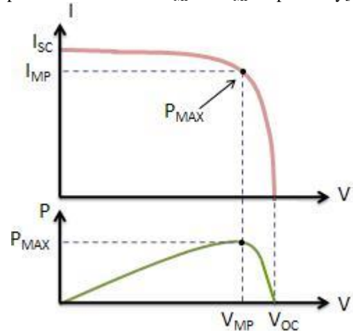
Figure 4 - Maximum Power for an I-V Sweep Fill Factor (FF)
