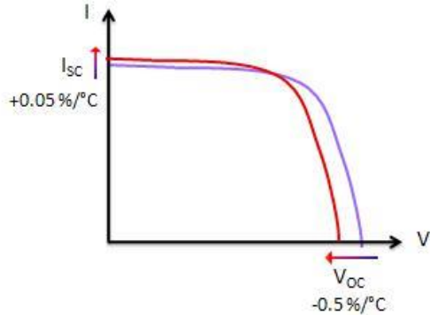
Figure 9 - Temperature Effect on I-V Curve
