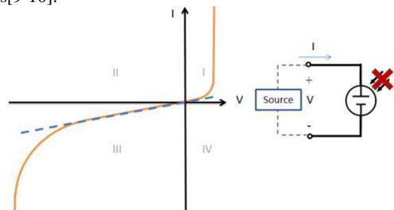
Figure 8 - I-V Curve of Solar Cell Without Light Excitation
