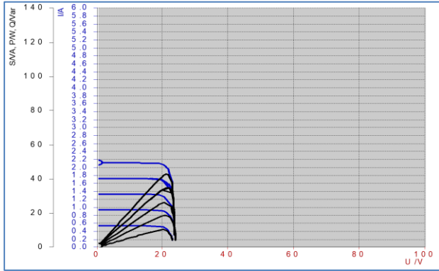
Figure 5 - Getting the Fill Factor From the I-V Sweep was taken “EPH 2 Advanced photovoltaics trainer”
