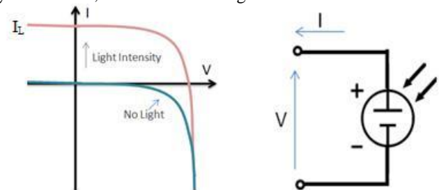
Figure 1 – I-V Curve of PV Cell and Associated Electrical Diagram
