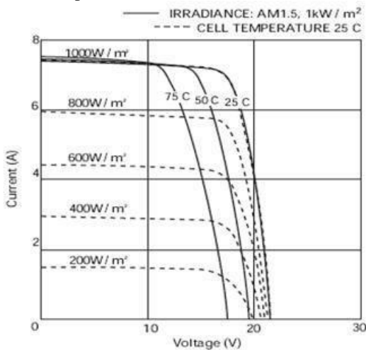
Figure 10 - Temperature Effect on I-V Curve I-V Curves for Modules
