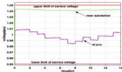
Voltage regulation by smart inverter with constant power factor (0.93)
