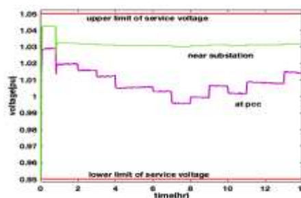
Figure (8) Voltage regulation by OLTC only caseI.1.
