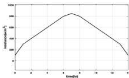
Figure(3) Solar raddiation during 14hour
