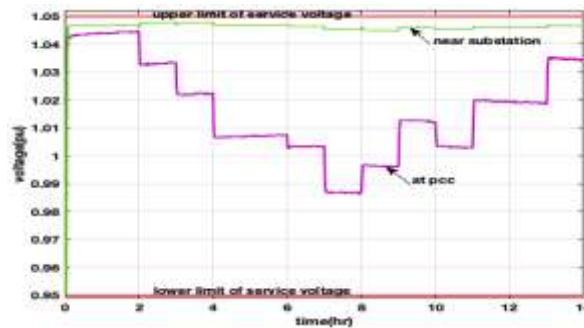
Voltage regulation by smart inverter with constant reactive power(400KVAR)
