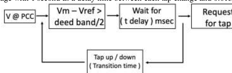
Figure(7) block diagram of OLTC
