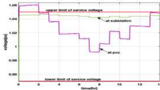
Voltage regulation by smart inverter with constant power factor (0.93)
