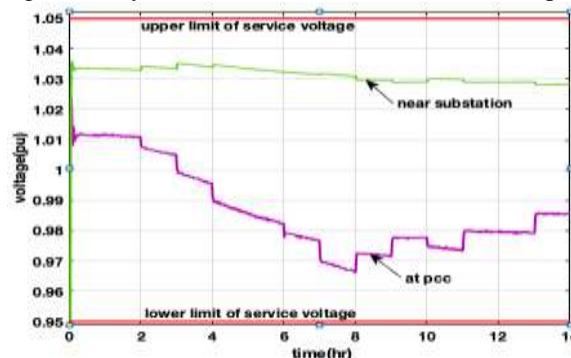
Voltage regulation by smart inverter with constant reactive power(400KVAR)
