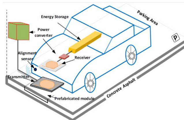
Figure 16 Static wireless electric vehicle charging system schematic.
