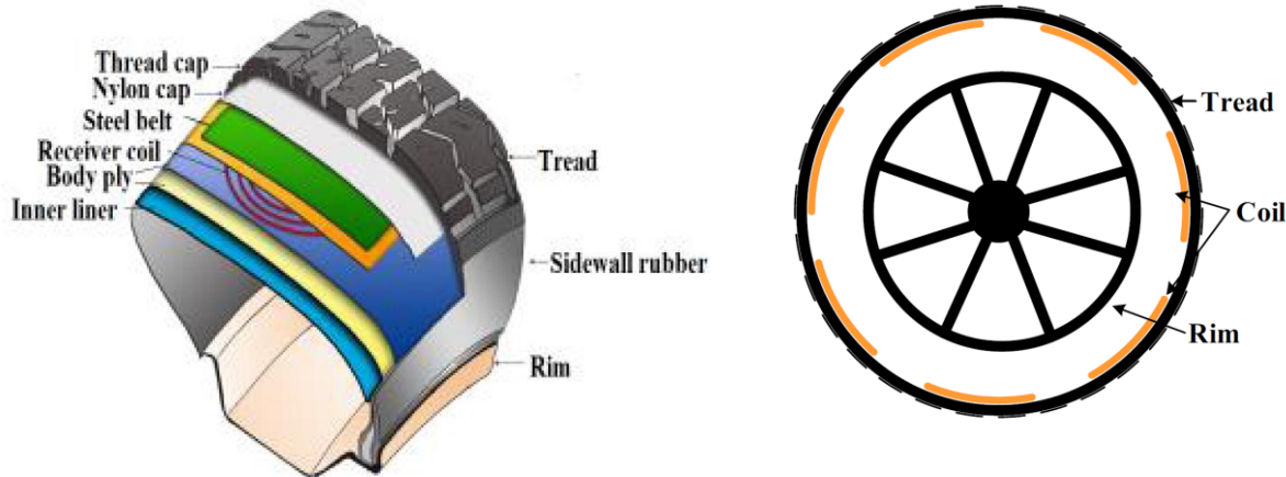
Figure 20 Internal coil positioning (a) and coil configuration (b) in the In-Wheel WCS.
