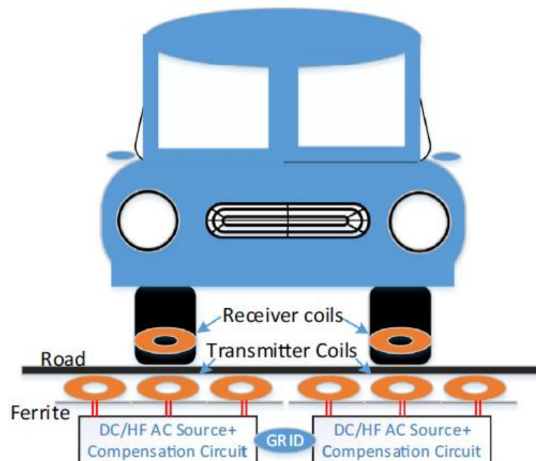
Figure 19 Static and Dynamic In-Wheel WCS Conceptual Illustration
