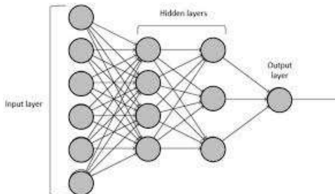
Figure 1: ANN Architecture
