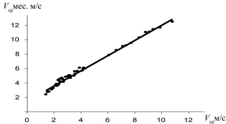
Fig 2. Dependence of the energy characteristics of the wind flow on the average wind speed
