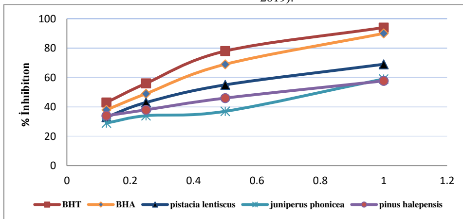
Figure 1- FRAP (ferric reducing antioxidant power)
