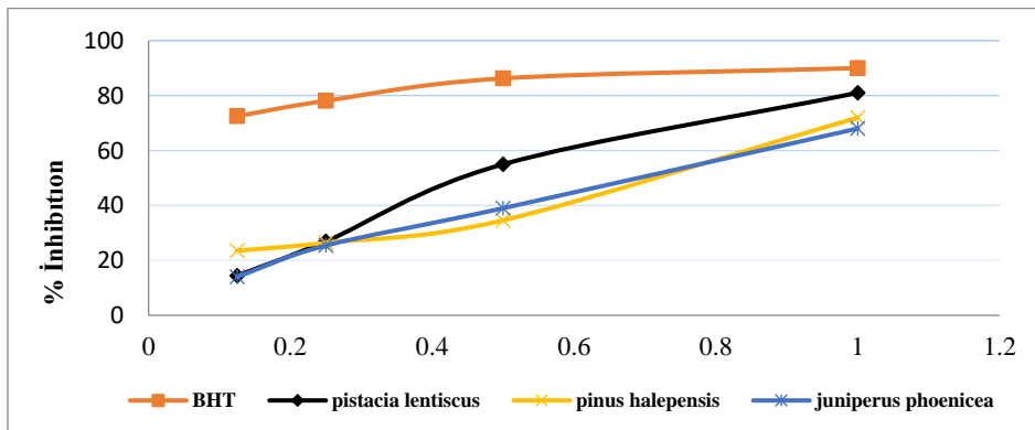
Figure 2- DPPH (radical scavenging activity)
