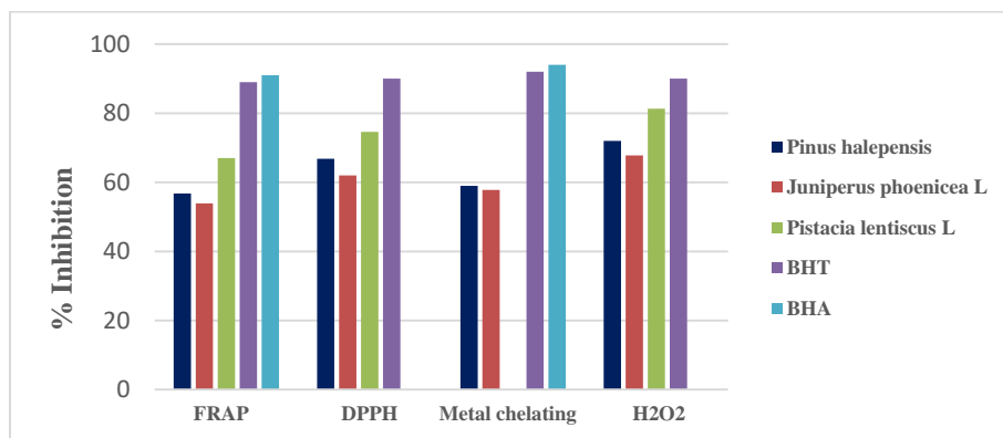
Figure.5- Radical Scavenging Capacity inhibition of bark samples
