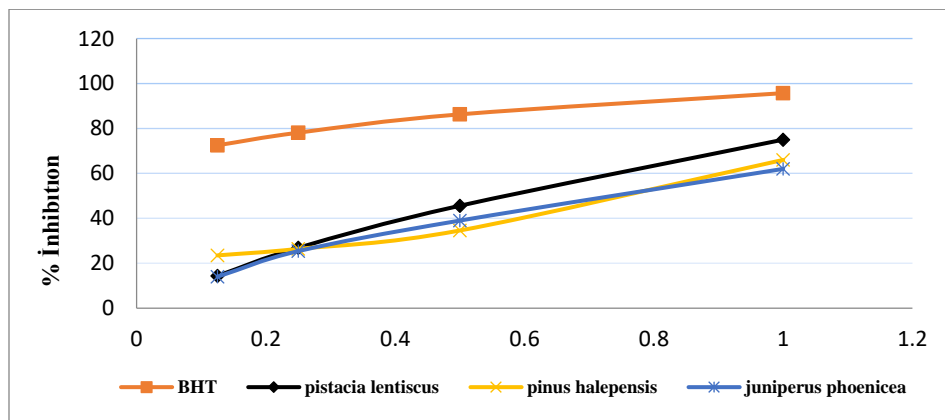
Figure 2- DPPH (radical scavenging activity)
