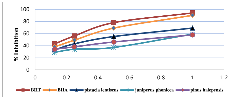
Figure 4- Metal Chelating Activities
