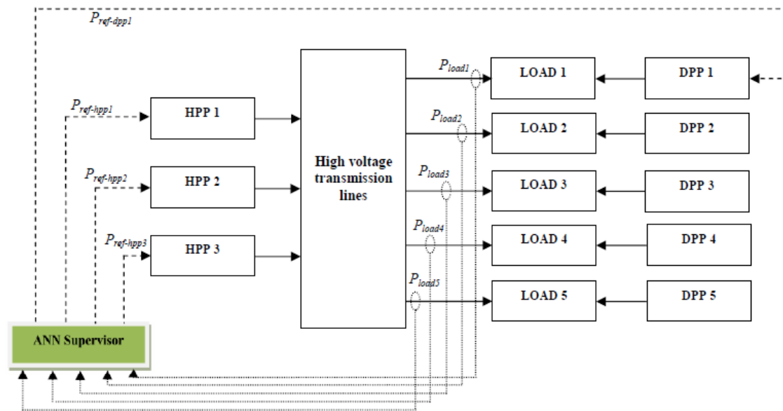
Fig. 1. Structure of IPS the region DIANA
