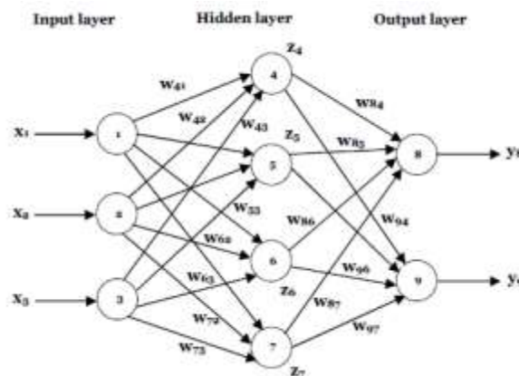
Fig. 4. Multilayer perceptron neural networks
