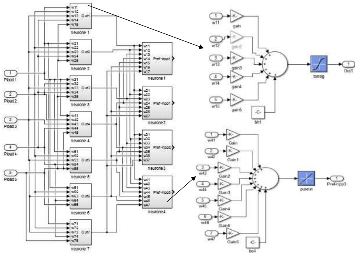
Fig. 8. Structure of the ANNS in Simulink
