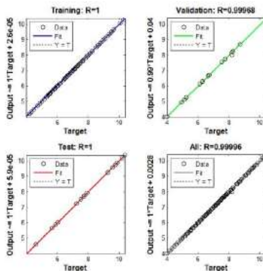
Fig. 6. Linear regression of the ANN (5-7-4)
