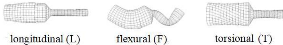
Fig 2 Mode shapes, from a finite element model of the ultrasonic horn
