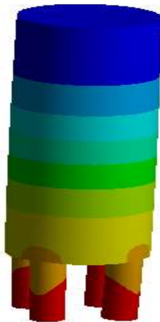
Fig 5: Harmonic response of vibrating horn
