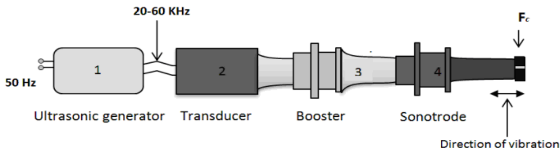
Fig 1 Main configuration of ultrasonic welding system
