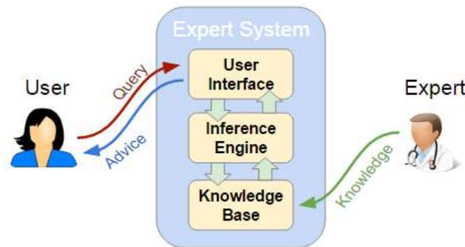
Figure 1: Expert system
