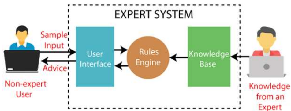
Figure 1: Expert system
