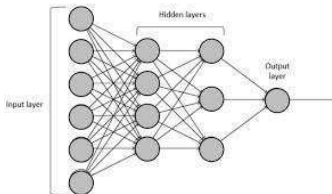
Figure 1: ANN Architecture
