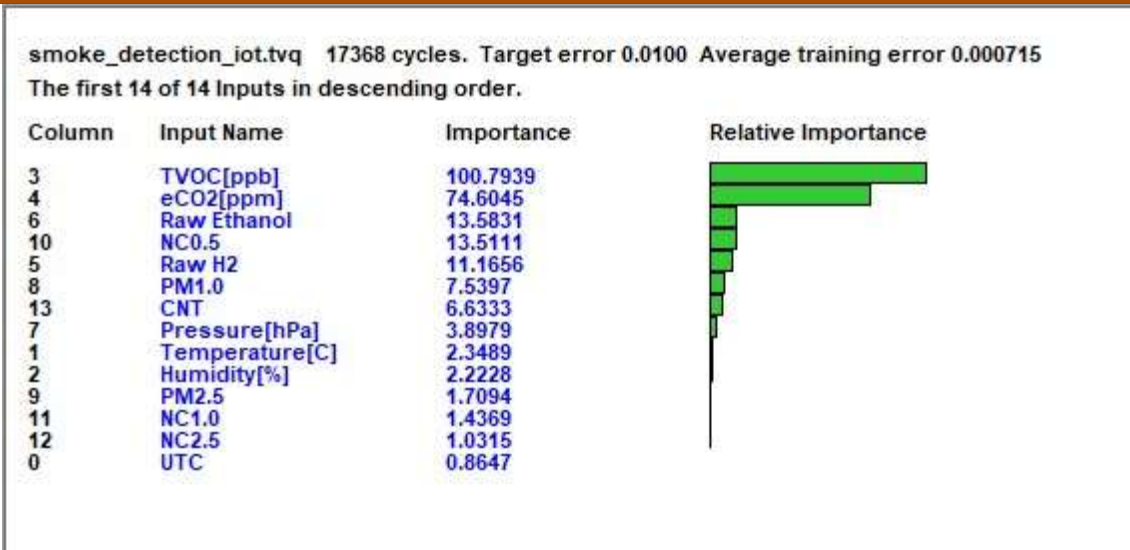
Figure 5: Most influential features in the dataset
