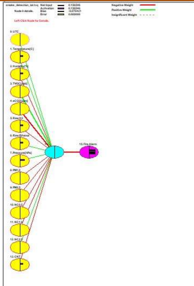
Figure 2: Structure of the proposed ANN model
