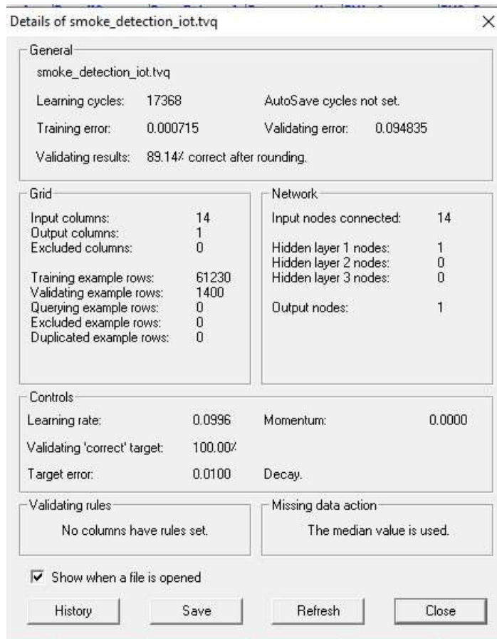
Figure 6: Details of the proposed ANN model
