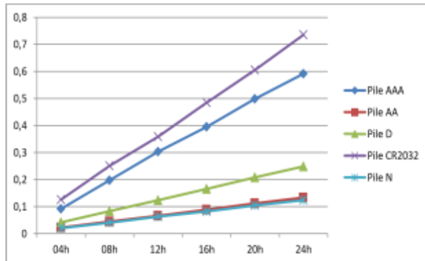
fig. 27. Representative curve of the tension drops of each pile tested.
