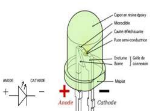
Fig. 3. Schematic and structural representation of an LED.
